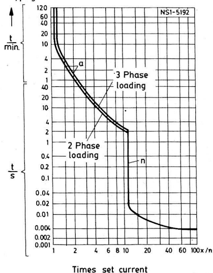
Time current characteristics of 3VU16
