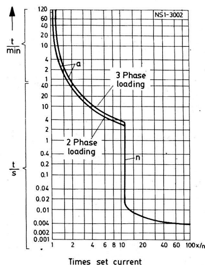
Tripping time
