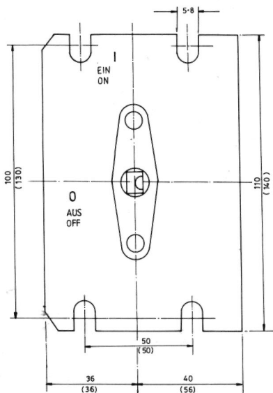
Mounting bracket of 3VU 13 / 16 3VU9133-1PA01 for 3VU 13 3VU9163-1PA02 for 3VU 16
